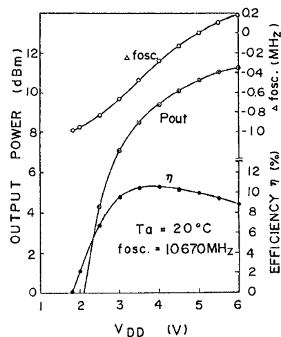
Fig. 16. Measured output power ( P_{out} ), oscillation frequency ( \Delta f_{osc} ) and efficiency ( \eta ) of dielectric resonator oscillator as a function of drain voltage ( V_{DD} ).
