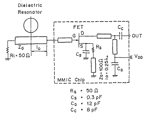
Fig. 8. Circuit diagram of dielectric resonator oscillator.
