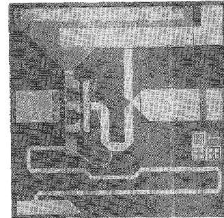
Fig. 9. Dielectric resonator oscillator chip ( 1.5 x 1.5 mm ).
