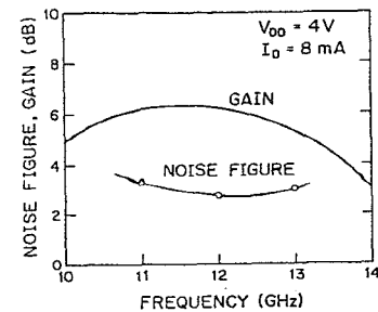
Fig. 11. Measured noise figure and gain of single-stage low-noise amplifier as a function of frequency.
