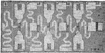
Fig. 5. Three-stage low-noise amplifier chip ( 1.5 x 3.0 mm ).
