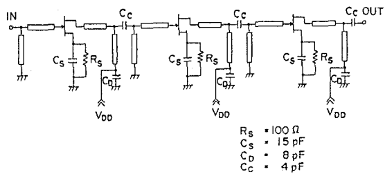
Fig. 4. Circuit diagram of three-stage low-noise amplifier.
