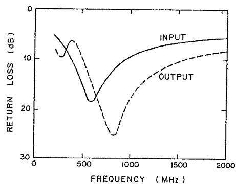
Fig. 15. Measured input and output return loss of 1 GHz IF amplifier as a function of frequency.
